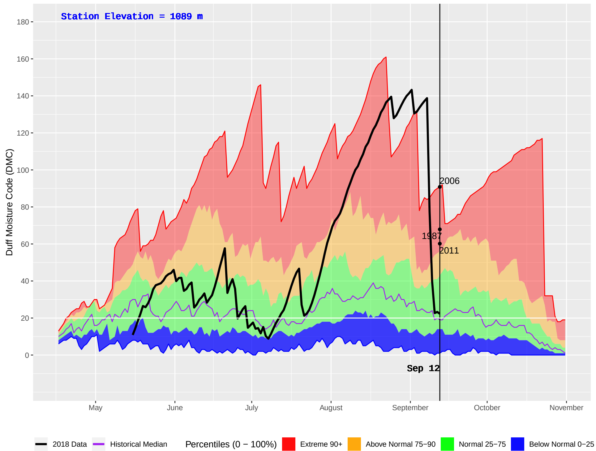
EAST OOTSA (170) : Historical (1986–2016) and Current (2018) Daily Duff Moisture Code (DMC)
