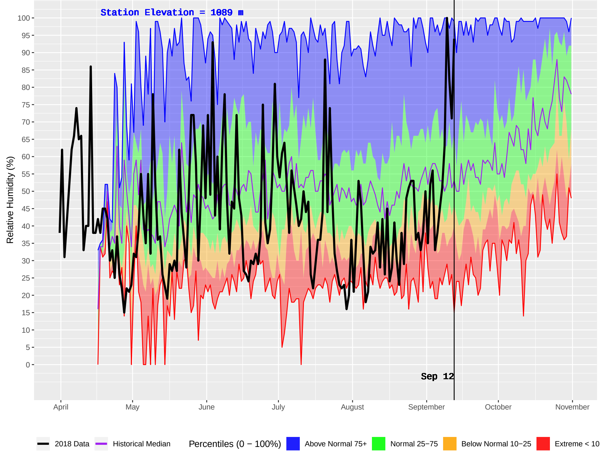
EAST OOTSA (170) : Historical (1986–2016) and Current (2018) Daily Relative Humidity
