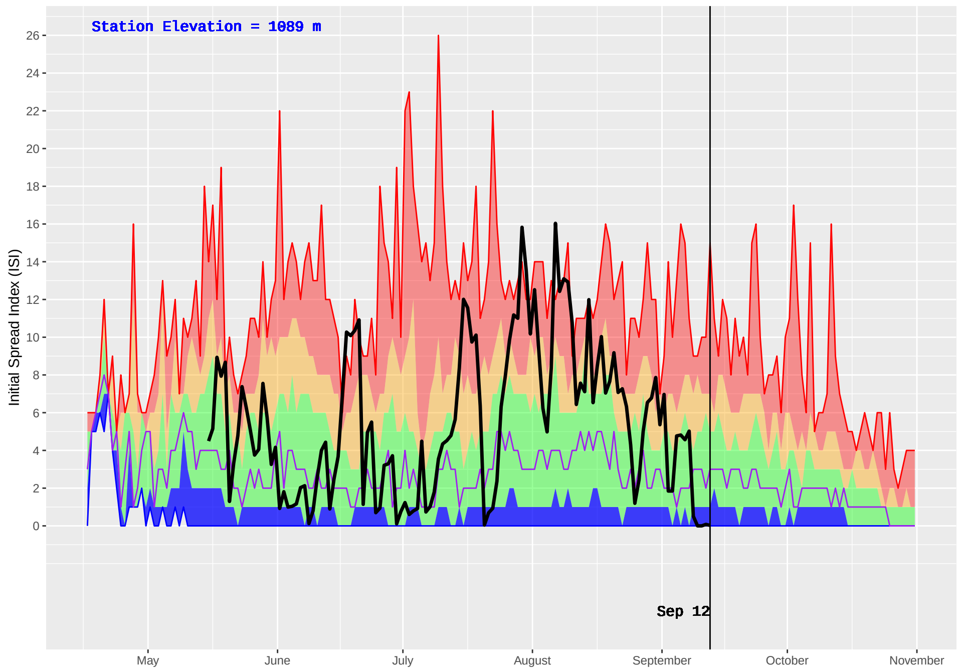
EAST OOTSA (170) : Historical (1986–2016) and Current (2018) Daily Initial Spread Index (ISI)
