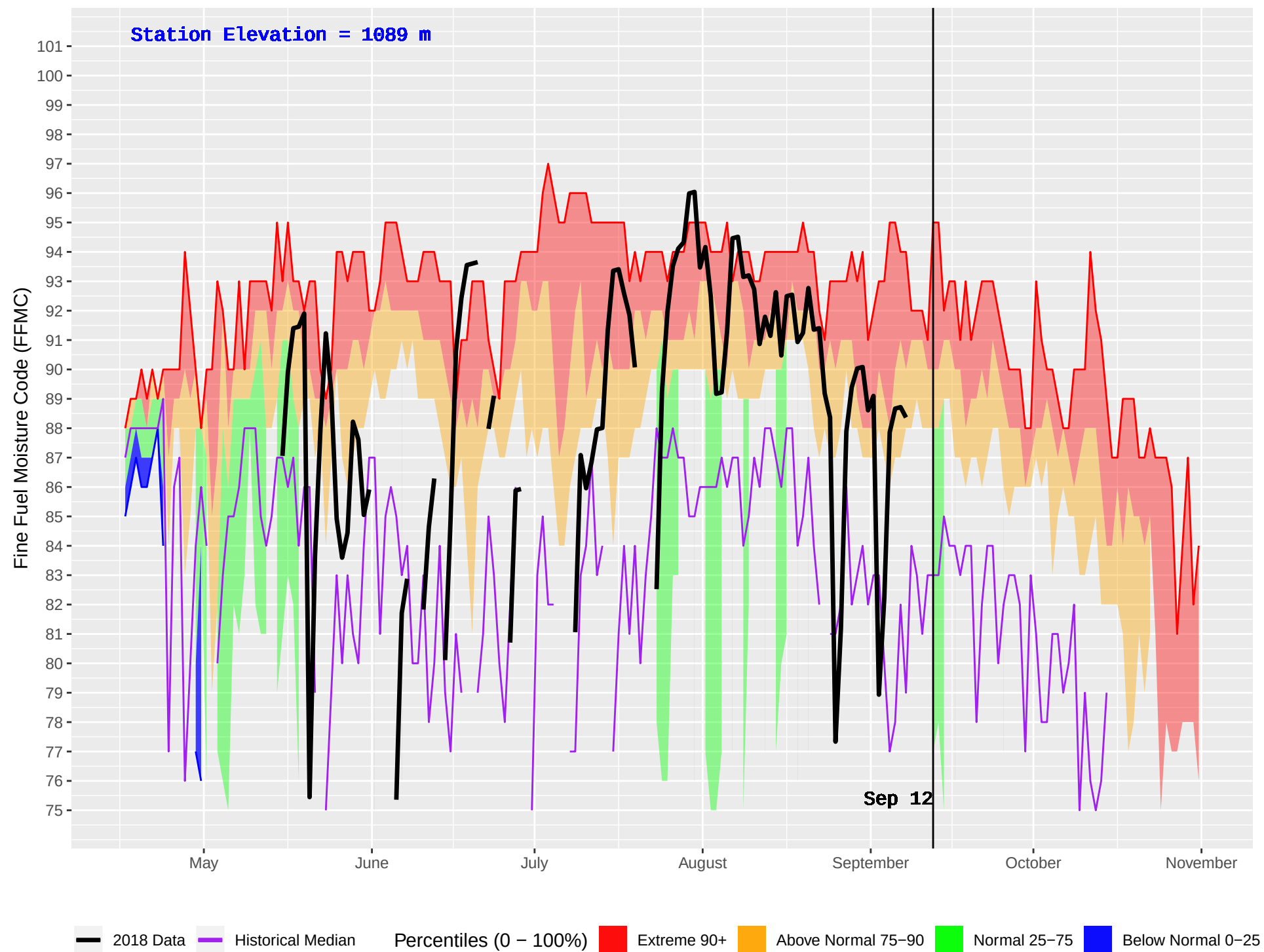
EAST OOTSA (170) : Historical (1986–2016) and Current (2018) Daily Fine Fuel Moisture Code (FFMC)
