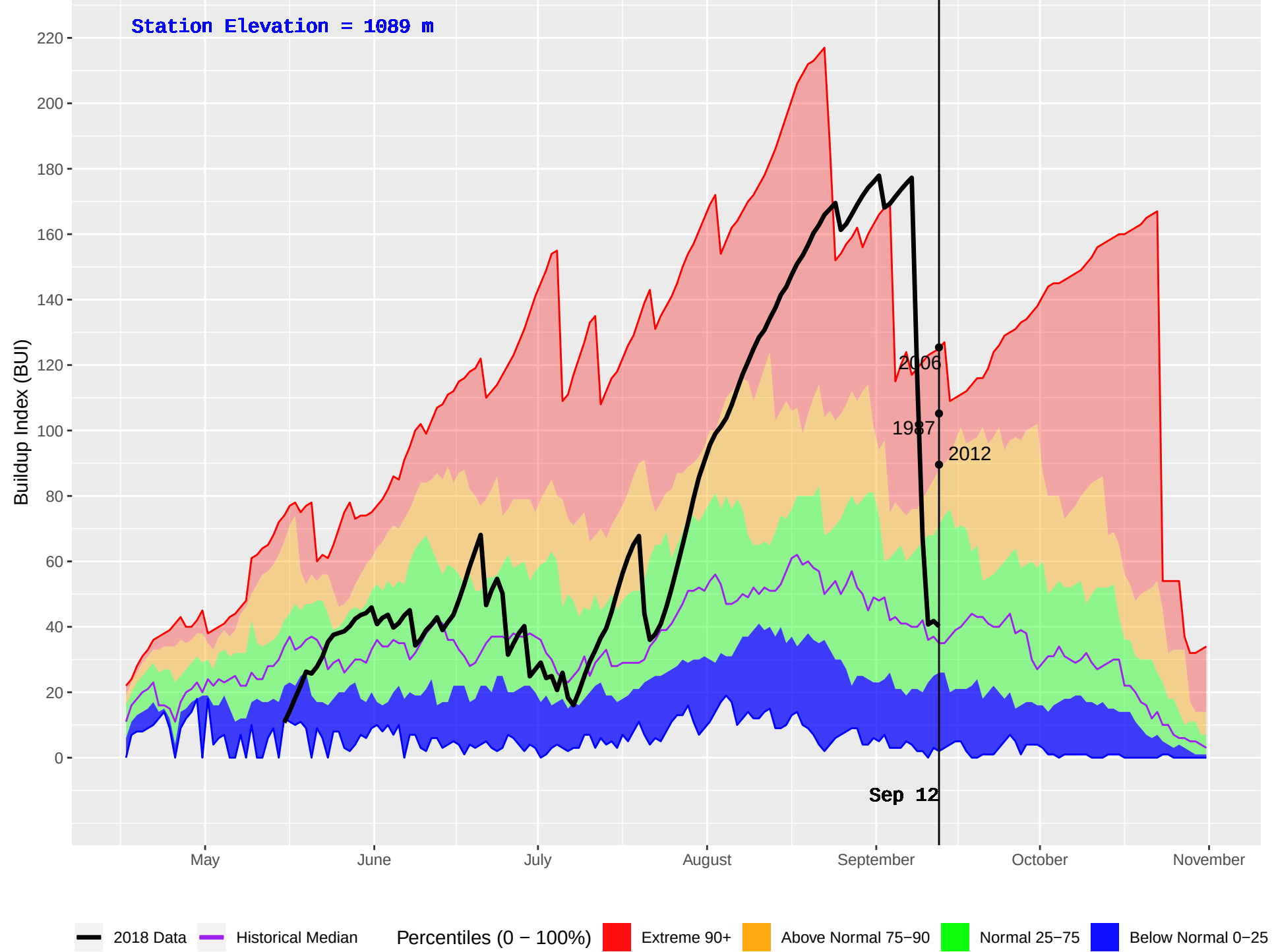
EAST OOTSA (170) : Historical (1986–2016) and Current (2018) Daily Buildup Index (BUI)
