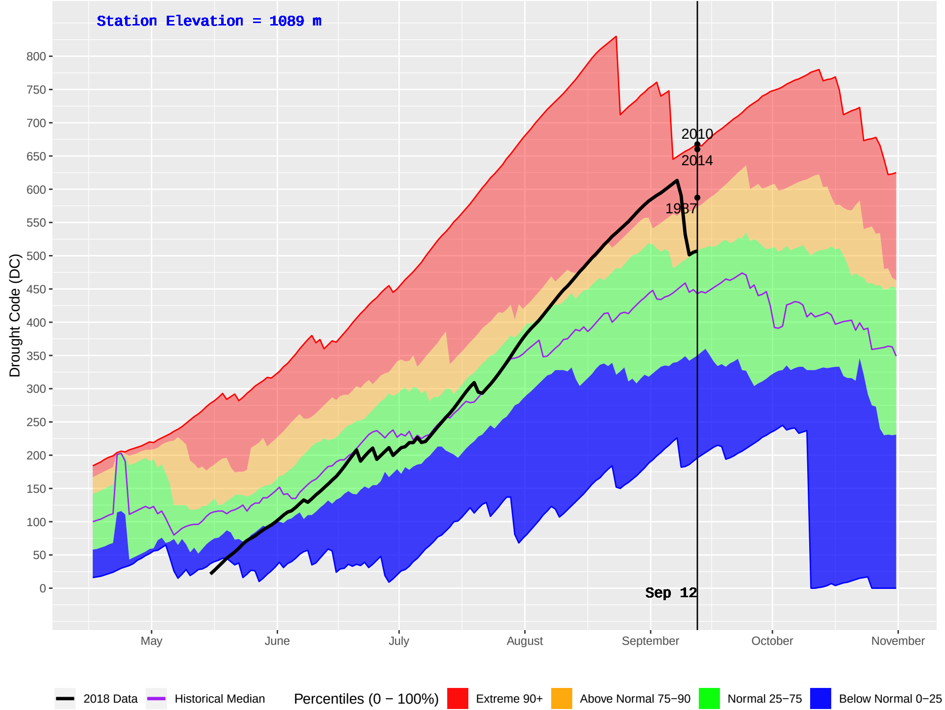
EAST OOTSA (170) : Historical (1986–2016) and Current (2018) Daily Drought Code (DC)
