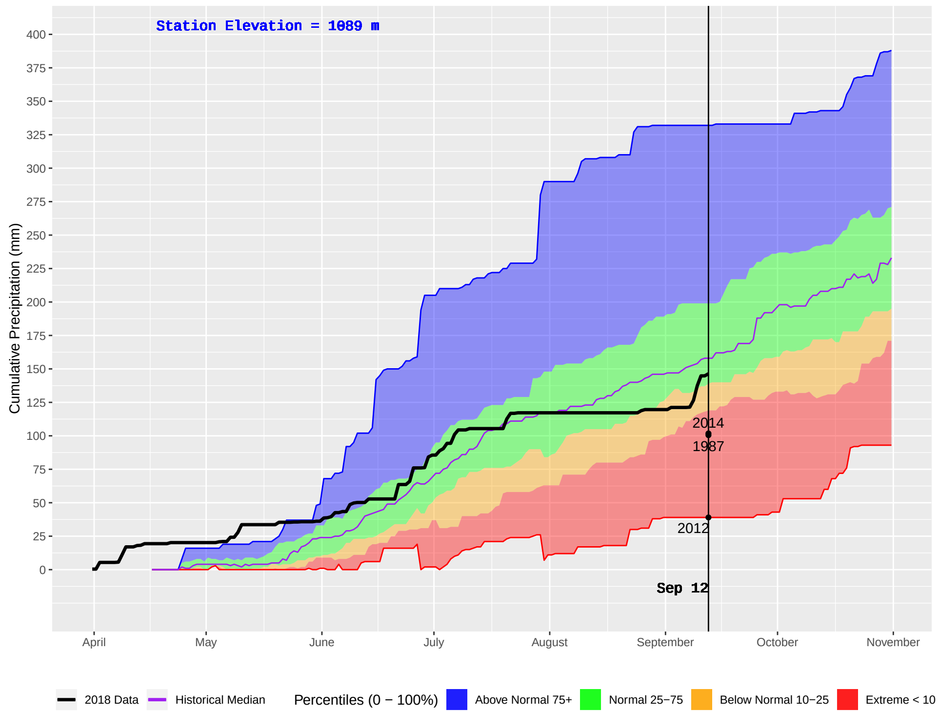
EAST OOTSA (170) : Historical (1986–2016) and Current (2018) Daily Cumulative Precipitation
